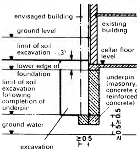
4 Section through underpinning → 5
